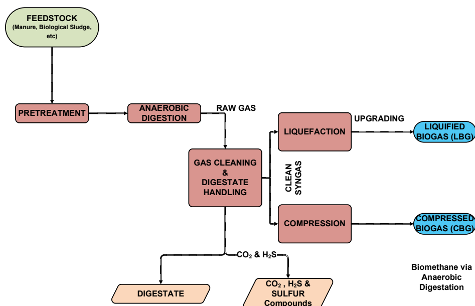
Figure 39 Simplified process flow diagram for biomethane from anaerobic digestion 104
