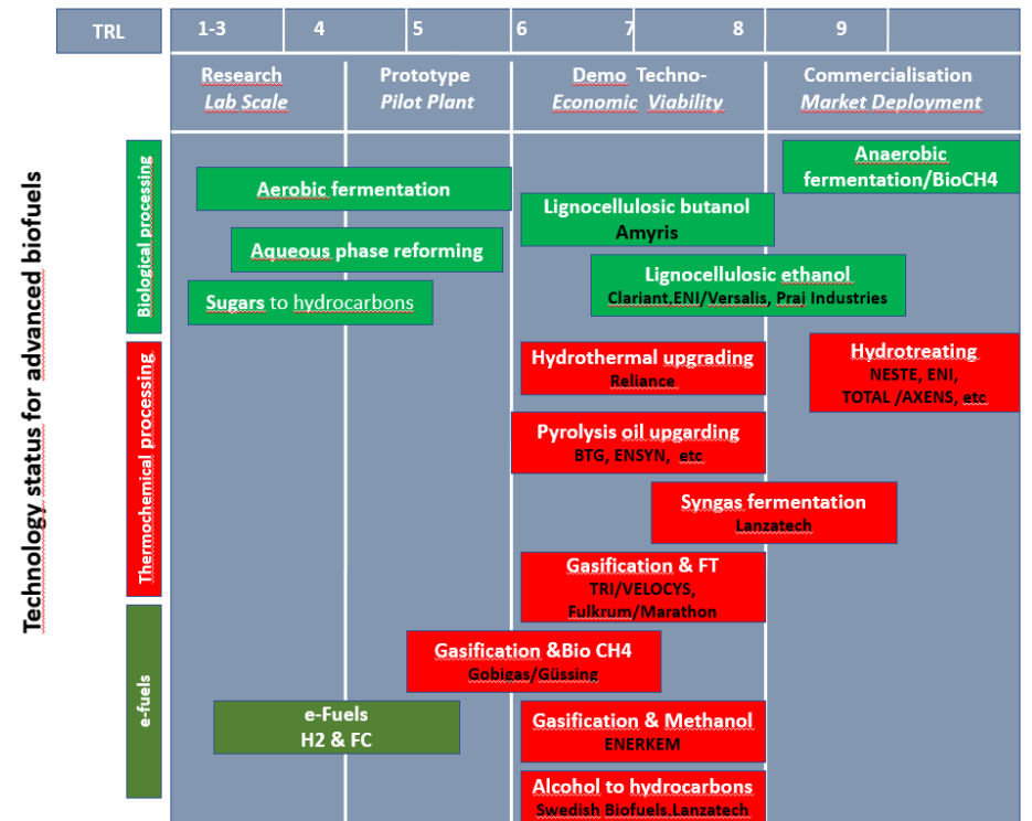
Figure 27: Status of advanced biofuels technologies based on their TRL level as well as their status based on the technology development roadmap
